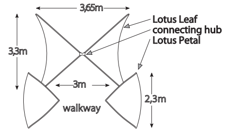
Plan View: one section of a Lotus Leaf Tunnel
